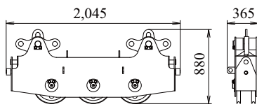
Upper Spreader (for Crane) Weight: 475 kg
