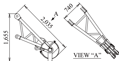
Auxiliary Sheave (for Crane) Weight: 275 kg
