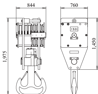
150 t Hook Weight: 2,300 kg
